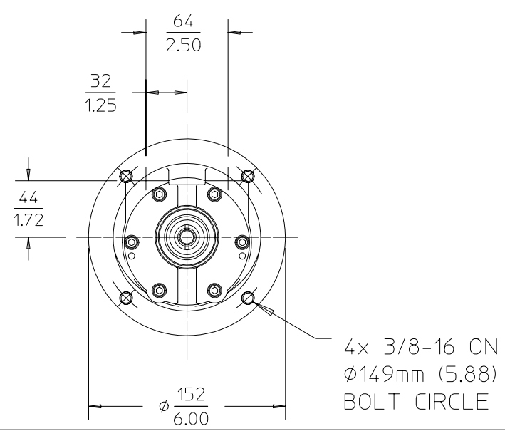
MUFFLER ASM. (SHIPPED UNATTACHED)
